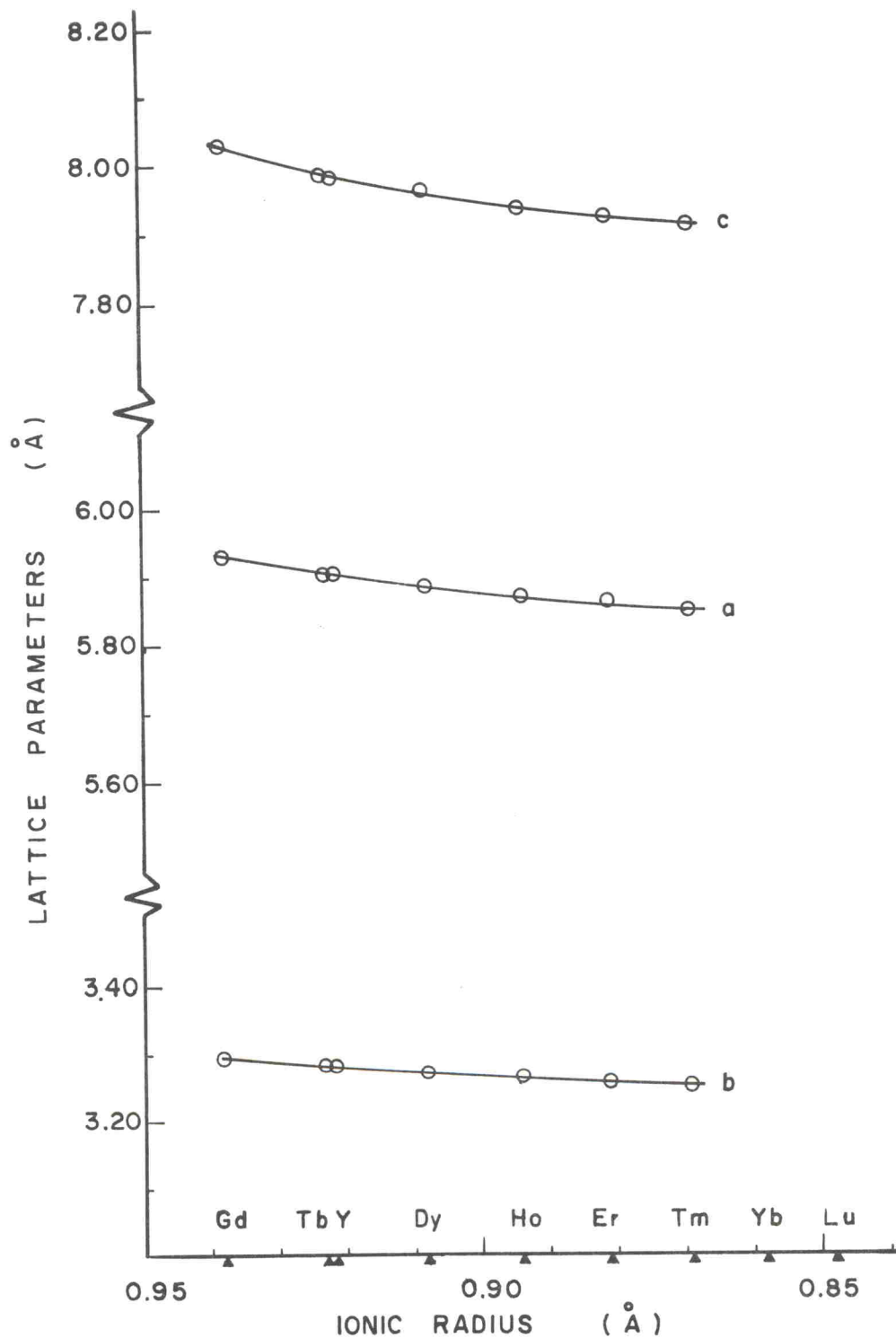
Fig. 21.--Variation of Lattice Parameters With Ionic Radius of High Pressure Orthorhombic Type Rare Earth Dioxides.
